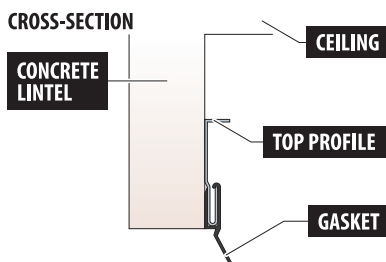
OPTION - Mounting the gasket on the lintel
