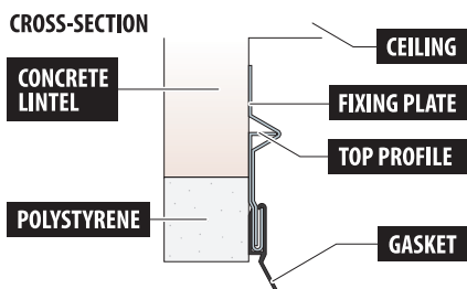
OPTION - Mounting the gasket on the lintel Lintel supported by polystyrene
