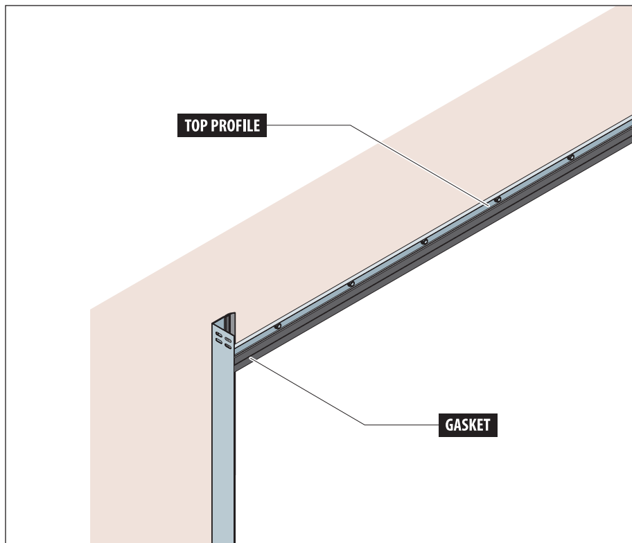
OPTION - Mounting the gasket on the lintel Lintel supported by polystyrene
